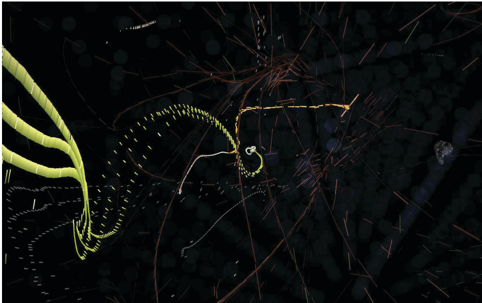
Figure 17-9. Higher-order orbital mixture of a hydrogen atom
