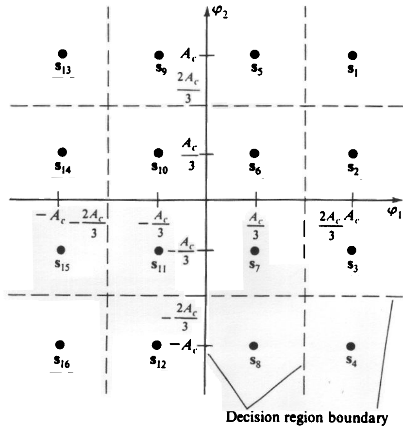
FIGURE 10.4.2 Optimum decision regions for equally likely 16-level QAM (Example 10.4.1).
