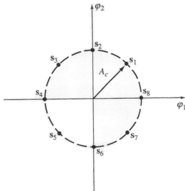
FIGURE 10.2.4 Signal space diagram for 8-phase PSK in Example 10.2.2.
