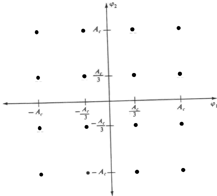
Signal space diagram for 16-level QAM (Example 10.2.1).
